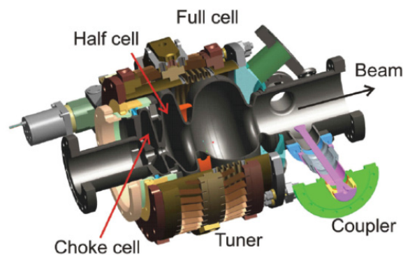
Figure 1: The SRF photoinjector for bERLinPro.
