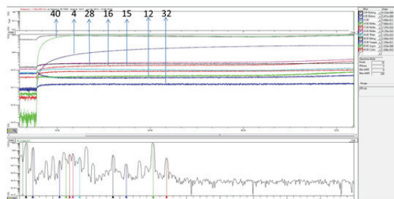
Figure 7: RGA trend after turning off ion pumps for build-up.
