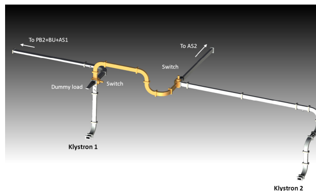
Figure 1: Modification of the RF distribution.
