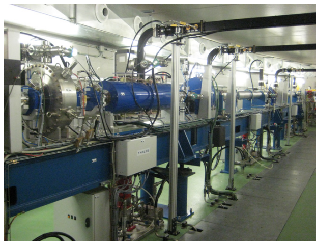
Figure 2: The ALBA Linac
