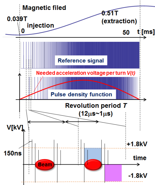
Figure 5: The acceleration voltages are generated discretely.
