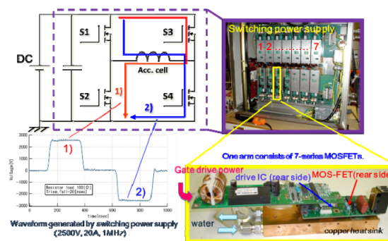
Figure 2: The schematic view of the induction acceleration system.
