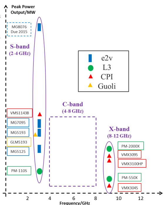
Figure 5: Magnetrons for X-ray screening arranged for clarity [14, 15, 16]. Please refer to device data sheets for definitive operating parameters.
