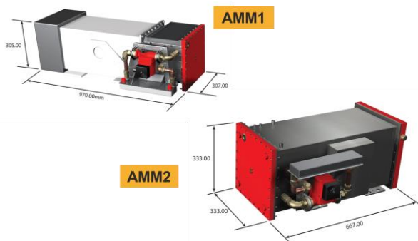
Figure 6: Displays e2v's solid state modulator range.
