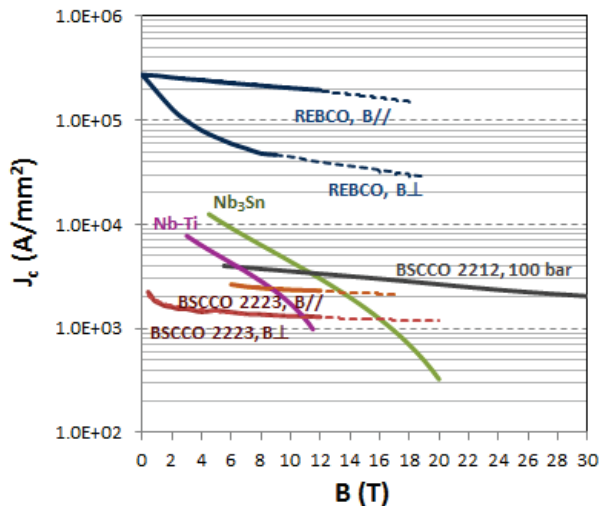
Figure 1: Critical current density ( J_c ) of superconductors in parallel ( B// ) and perpendicular ( B\perp ) magnetic field ( B ). Values for BSCCO 2212 are from [7], BSCCO 2223, REBCO and Nb_3Sn curves are from measurements at 4.2 K performed at CERN on commercial materials. The LHC Nb-Ti curve is at 1.9 K.
