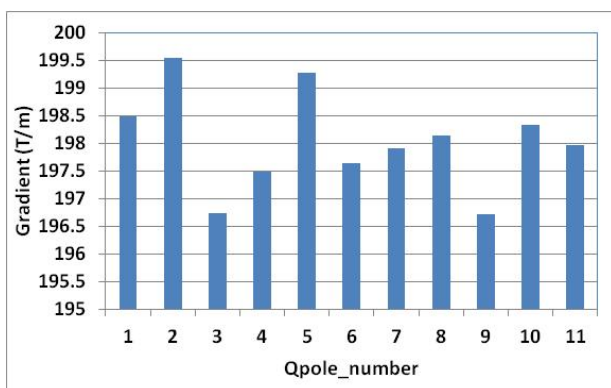
Figure 6: PMQs measured gradient values (Rrif=1 mm).
