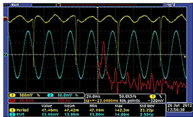
Figure 4: Measurement at R=1mm on PMQ #8 (oscilloscope screen).
