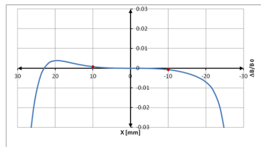
Figure 6: Field tolerance of ILSF quadrupole magnet boundaries of the good field region ( \pm 10 mm) are shown in red.
