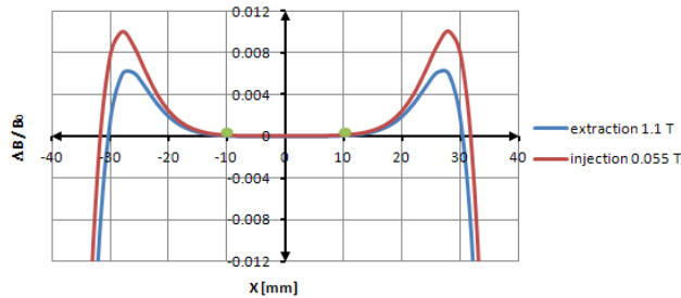
Figure 3: ILSF dipole field tolerances, red line is for injection at 0.055T and , blue line indicates extraction field tolerances at 1.1T .
