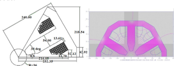
Figure 7: Magnetic field lines and geometry of the sextupole magnet in ILSF.
