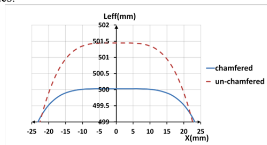
Figure 5: Effective length for a 483 mm long quadrupole before and after chamfering.
