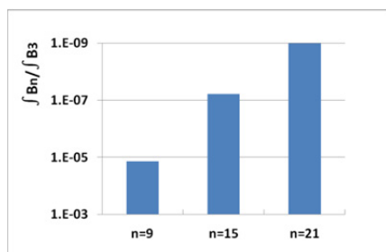
Figure 9: Normalized integral field harmonics for a sextupole in ILSF.
