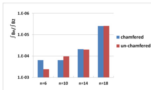
Figure 6: Normalized integral field harmonics for the chamfered and un-chamfered quadrupole.
