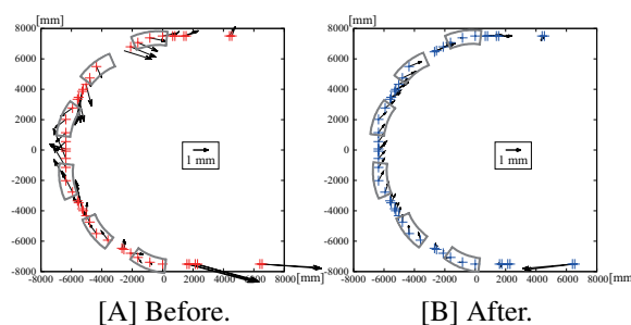
Figure 5: Magnet positions in ARC plane. A is before realignment, while B is after. Vectors are differences between magnet positions and design values. Gray boxes show BMs.
