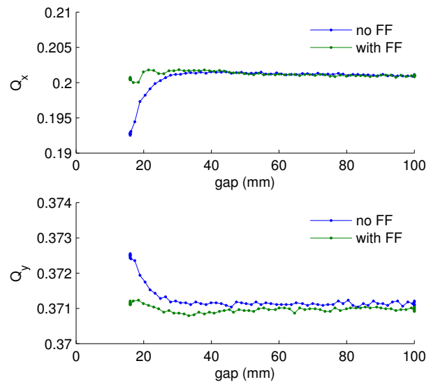
Figure 3: Tune shift with gap for J09 (vertical polarisation).
