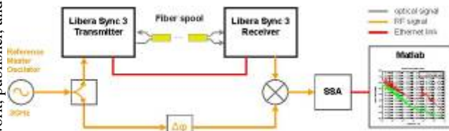
Figure 2: Jitter measurement setup.
