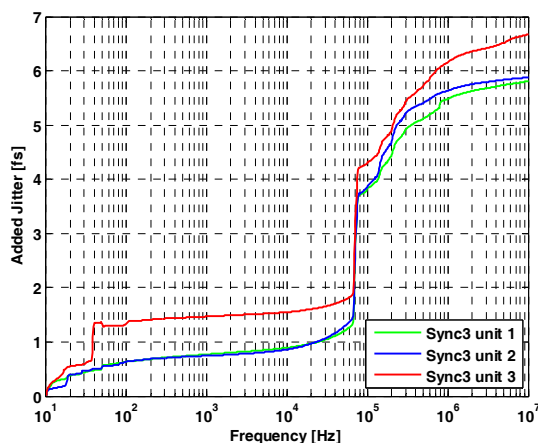
Figure 4: Added jitter.
