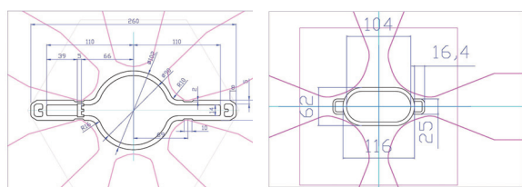
Figure 1: Typical cross-section of beam pipes in SuperKEKB. Left: LER with antechamber at arc sections in a sextuple magnet. Right: HER with race-track shape at the arc sections in a quadrupole magnet.
