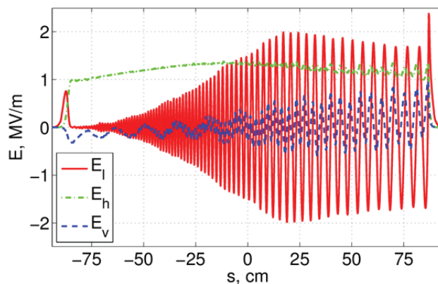
Figure 4: On-axis field components in LANL RFQ.
