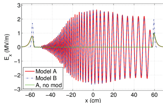
Figure 2: On-axis longitudinal field in FNAL RFQ.
