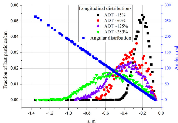
Figure 3: Longitudinal and angular distributions of the lost particles during the steady-state-loss quench test, with different ADT gains.
