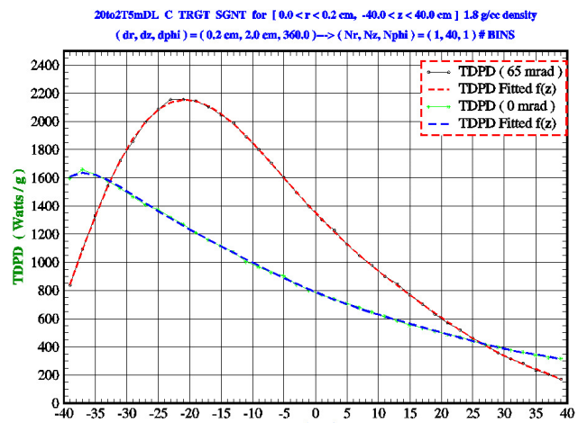
Figure 7: Power deposition on the axis of targets tilted at 0 and 65 mrad, for a 4-MW proton beam.
