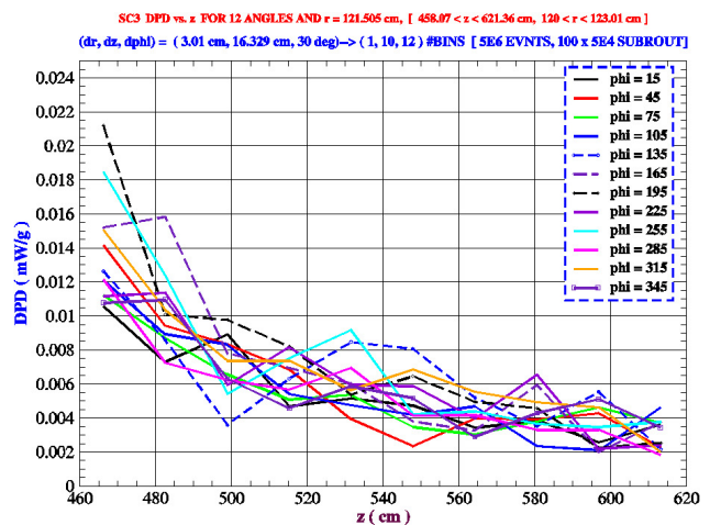
Figure 5: Power deposition in superconducting coil 3 as a function of z , for 12 bins of 30^\circ in azimuth, for 4-MW proton beam power.
