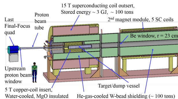
Figure 1: Sketch of the Target System concept, including the second magnet module that completes the field taper from 20 T on the target down to 2 T in the Decay Channel.
