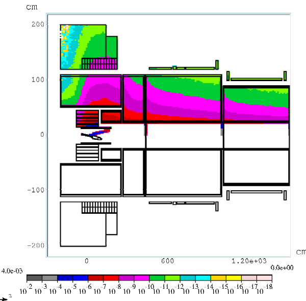
Figure 3: Simulated power deposition in the Target System for a 4-MW proton beam, averaged over azimuth.
