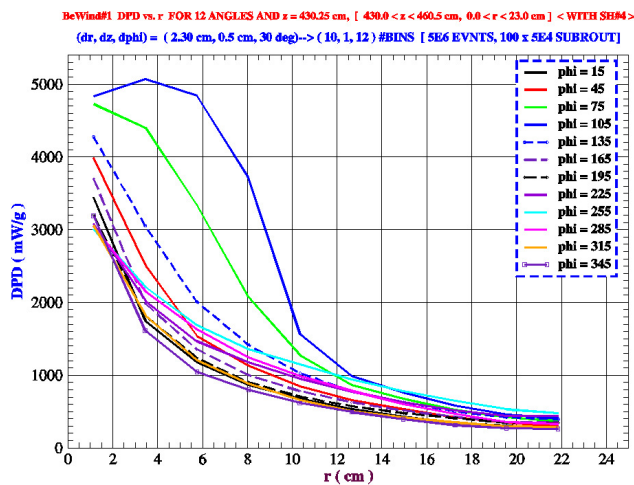
Figure 6: Power Deposition in a 2.5-mm-thick Be window at z = 430 cm, for 4-MW proton beam power.
