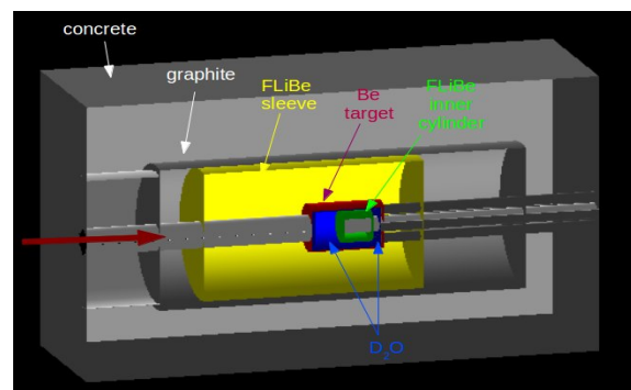
Figure 4: Current design of the ISODAR target with the surrounding components (moderator, sleeve, reflector and shielding).
