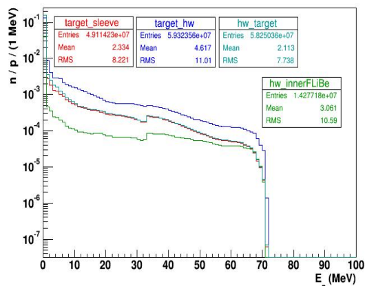
Figure 6: Neutron spectra for neutrons crossing the barrier components.
