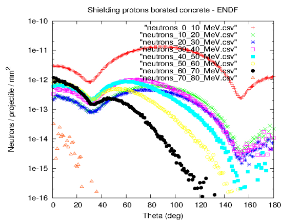
Figure 2: The number of neutrons per mm^2 escaping the 500 mm thickness shielding normalised to the incoming protons. The material used in this calculation is borated concrete.
