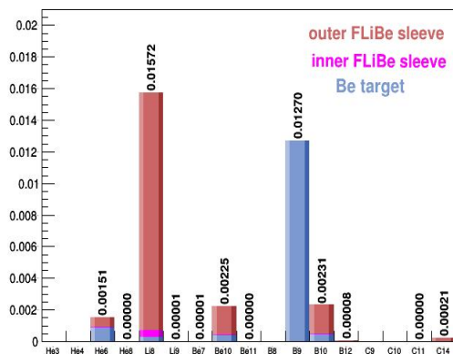
Figure 5: Total isotopes production in the Be vessel and FLiBe components. Different colours represent the contribution to the isotope yield from target, inner FLiBe disk and FLiBe sleeve.
