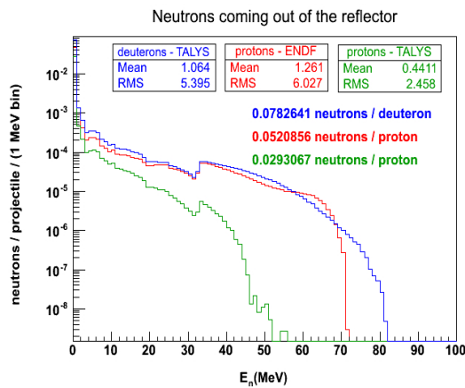
Figure 1: Comparison between the neutron spectra out of the graphite reflector for protons and deuterons projectiles. For protons, the cross sections were calculated with both experimental data and theoretical models.
