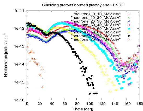
Figure 3: The number of neutrons per mm^2 escaping the 500 mm thickness shielding normalised to the incoming protons. The material used in this calculation is borated polyethylene.
