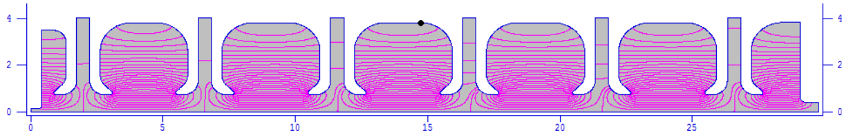
Figure 3: The field distribution of the whole accelerating tube.
