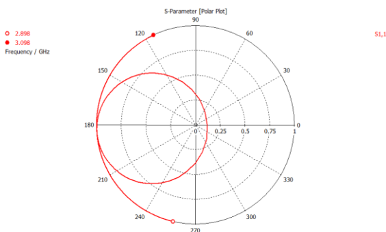
Figure 10: Smith Chart of Coupler.
