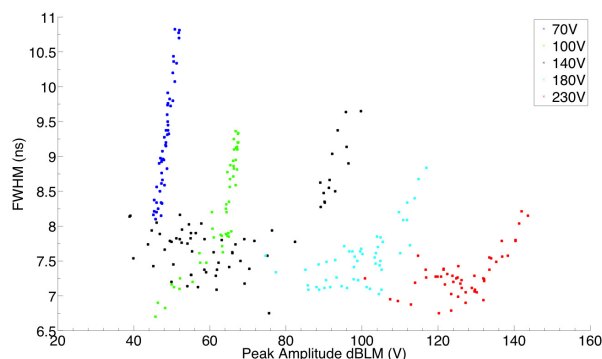
Figure 9: FWHM vs. peak amplitude of the dBLM signal.
