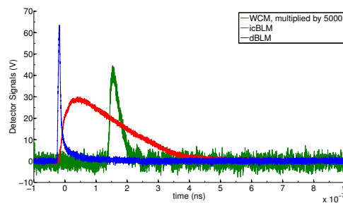
Figure 4: Signals of the three detectors. The dBLM signal is marked in blue, icBLM in red and the signal of the WCM in green. The signal of the WCM is multiplied by 5000 for a better visibility.
