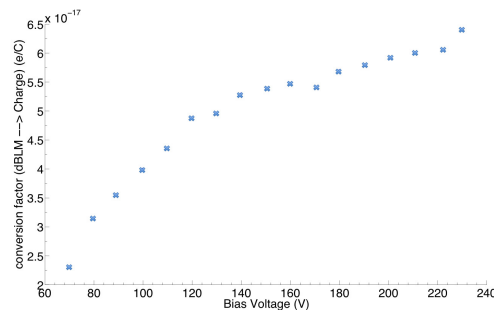
Figure 6: Factors (e/C) to convert dBLM signal in Coulomb to the numbers of particles for different bias voltages.
