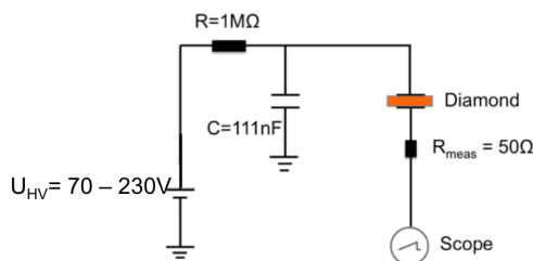
Figure 1: Circuit diagram of a diamond detector. The bias voltage was 70-230V, the diamond was connected to a 50 Ohm terminated read-out system.
