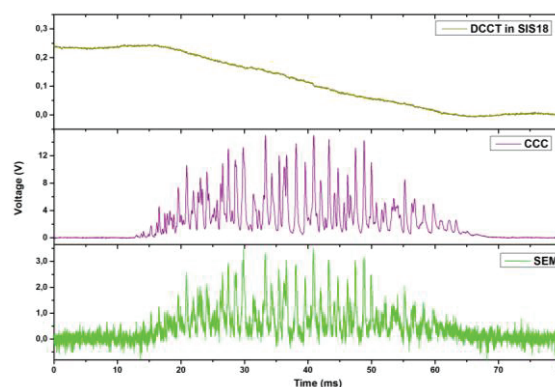
Figure 2: Slowly extracted \text{Ni}^{26+} beam measured with DCCT (top), CCC (middle) and SEM (bottom).
