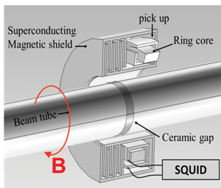
Figure 1: CCC schematic setup.
