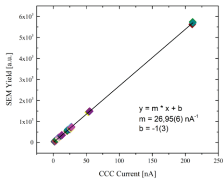
Figure 3: SEM signal as function of beam current measured with the CCC (note the small error of slope m ).
