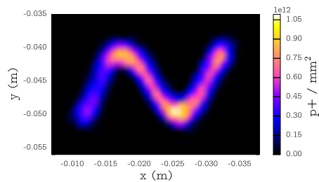
Figure 2: Particle density on the TIDVG front face for HL-LHC beam parameters (Table 1).
