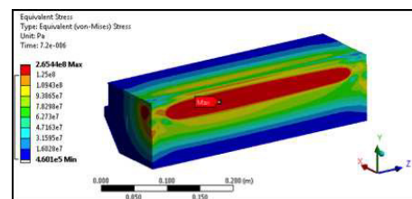
Figure 4: Von Mises stresses in aluminium block with HL-LHC energy deposition. Red parts are overstressed (>125 MPa). Only half of the block is represented.
