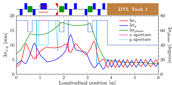
Figure 2: Schematics layout of the MEBT lattice (top), beam envelopes ( 3\sigma ), and apertures. In the schematic, blue boxes are quadrupoles, green boxes are buncher cavities, red lines are chopper plates, and red triangles are a chopper dump.
