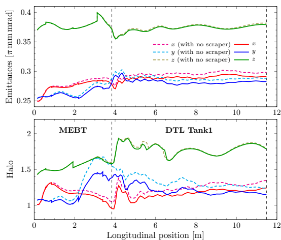
Figure 4: Evolutions of emittances (top) and halo parameters (bottom) in the MEBT and the first DTL tank.
