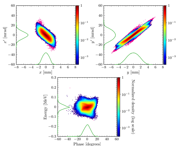
Figure 5: Particle densities at the MEBT exit. Magenta points represent additional particles in case of no scraper.
