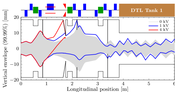
Figure 3: Vertical envelopes (99.99%) for the chopper voltages of 0, 1, and 4 kV cases.
