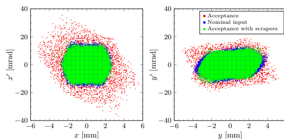
Figure 6: Acceptances of the transverse planes at the MEBT entrance with and without the scrapers.
