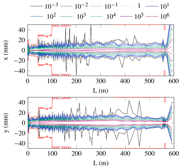
Figure 1: Power density levels from the RFQ exit to the target. The beam power outside of the outermost line is 1 \times 10^{-3} W. Red line shows the beam aperture.
