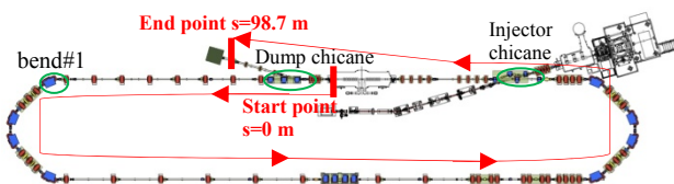
Figure 1: The cERL beam line used for tracking simulations.
