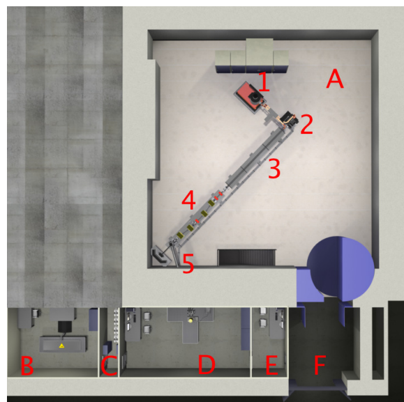
Figure 1: Layout of the FLUTE building. Bunker (A): klystron with auxiliaries (1), gun with solenoid (2), linac (3), bunch compressor (4), THz beam line (5), laser clean room (B), airlock (C), experimental room (D), control room (E), entrance area (F).
