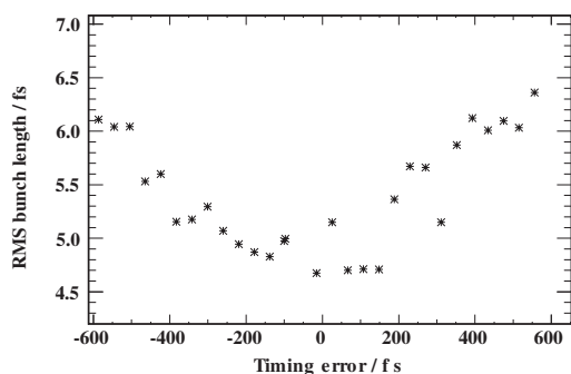
Figure 2: RMS bunch length as function of the timing error for a 1 pC bunch. The bunch length increases significantly for timing errors larger than \pm 200 fs and shows fluctuations in the order of 0.5 fs around zero.
