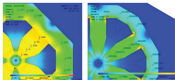
Figure 10: Saturation field map for quadrupole and sextupole.
