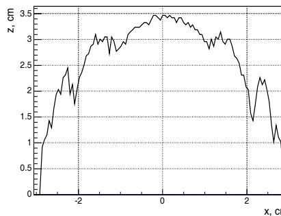
Figure 6: DA of the 10 pm emittance storage ring at \beta_{x,y} = 10 m
