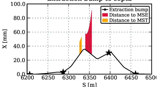
Figure 8: Extraction bump and septa for LSS6 extraction of LHC beam 1. The distance of the bump to the MST varies between 18 and 22 mm and 23 to 63 mm to the MSE.
