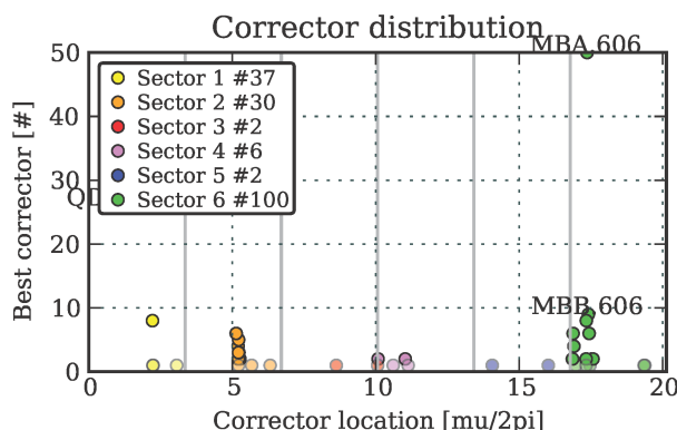
Figure 6: The best corrector for this period is the dipole MBA.606, followed by QD.133 and MBB.606.
