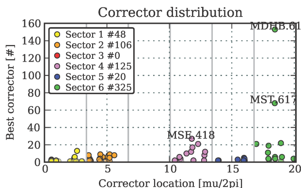
Figure 4: For the first period the MST.617 and MDHB.61804 show up as the main correctors.
