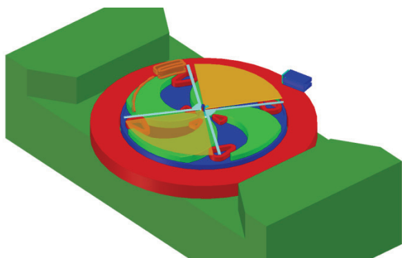
Figure 1: Half cut model of the cyclotron NIRS-930.
