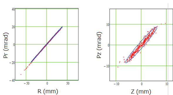
Figure 3: The phase space plot of the extracted beam in simulation.
