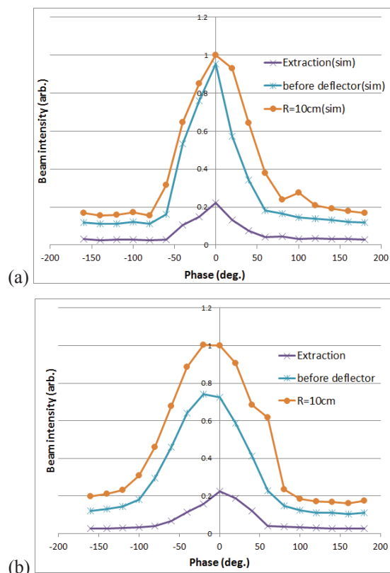
Figure 4: Beam intensity of each part of the cyclotron as functions of RF phase in the case of (a) simulation and (b) experiment. Ordinate is beam intensity of arbitrary unit where the intensity at R=10cm is defined as 1.
