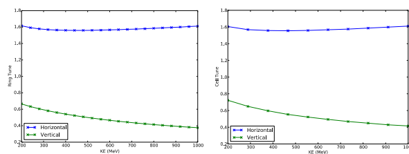
Figure 3: Machine tunes for the 2m ring (left) and the mini-racetrack FFAGs (right) as a function of beam energy.
