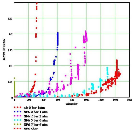
Figure 2: Corona current versus voltage.
