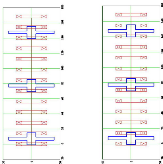
Figure 4: Conceptual design magnet system for 8 MV cooler.
