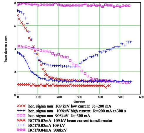
Figure 1: The beam size and proton beam intensity versus time for cooling experiments at different energies COSY.
