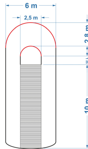
Figure 3: Conceptual design of the voltage vessel for 8 MV cooler.
