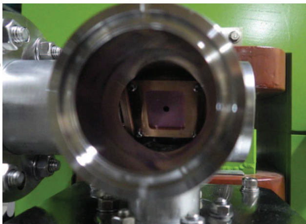
Figure 2: Beam spoiler has been installed in the linac beam line. The hole aperture is 3 mm.
