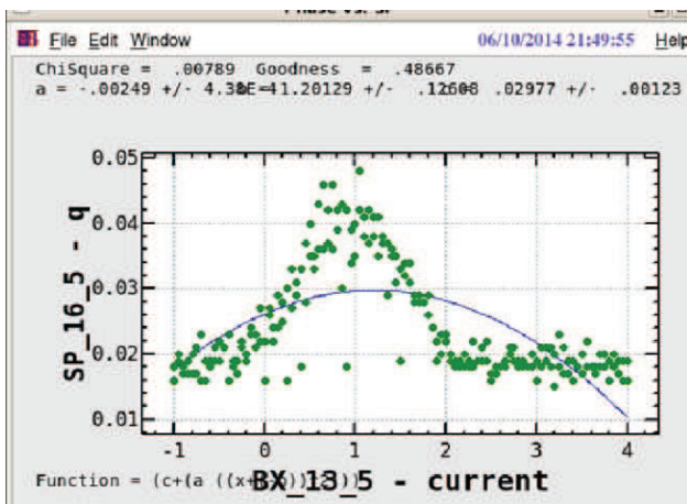
Figure 6: BMP( SP_{16_5} ) measurement of positron charge as a function of the steering ( BX_{13_5} ) current. Primary electron beam was scattered by the beam spoiler.
