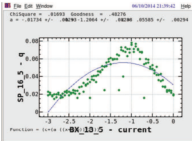
Figure 5: BMP( SP_{16_5} ) measurement of positron charge as a function of the steering ( BX_{13_5} ) current. Primary electron beam passed through the spoiler center hole.
