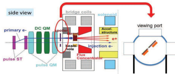
Figure 1: Schematic view of SuperKEKB positron source configuration and spoiler principle design.
