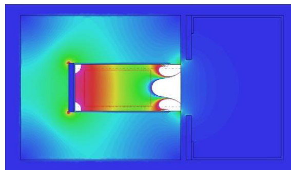
Figure 2: MKP-I simulated B-field with indicated good field region (red line). White areas are outside ±0.5%.
