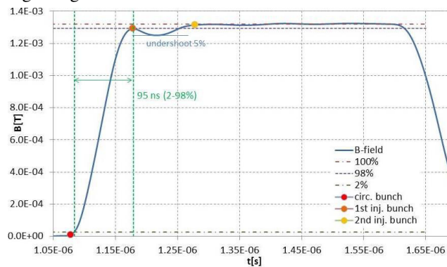
Figure 4: B-field of MKPS magnets connected to a PFL.
