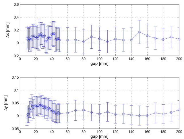
Figure 2: Electron beam position as a function of the gap of the first sFLASH-undulator at a BPM downstream.
