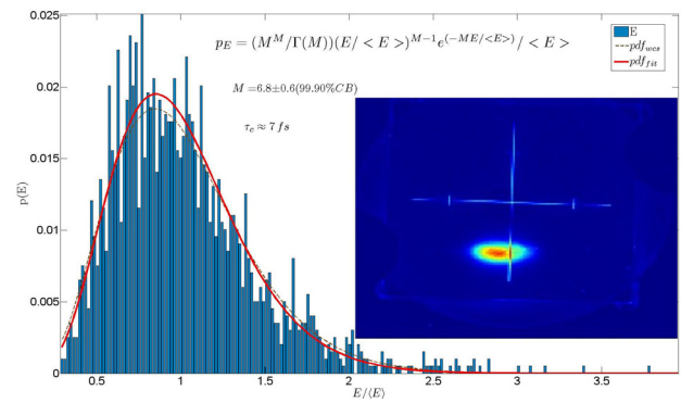
Figure 6: Probability distribution of the energy in the SASE-pulses and transverse profile of the SASE radiation on the YAG screen (inset).
