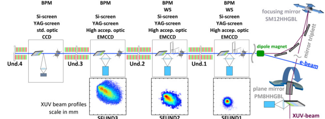
Figure 3: The schematic of the sFLASH beamline. It illustrates the injection beamline for the seed laser and the beam diagnostic stations. Exemplary XUV beam profiles along the undulator using a mirror with a focal length of 6.25 m are also shown [3].
