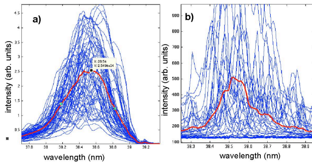
Figure 5: (a) Single-shot spectra of the SASE-radiation. (b) Single-shot spectra of the HHG seed. The red curve is the average over all single shots.
