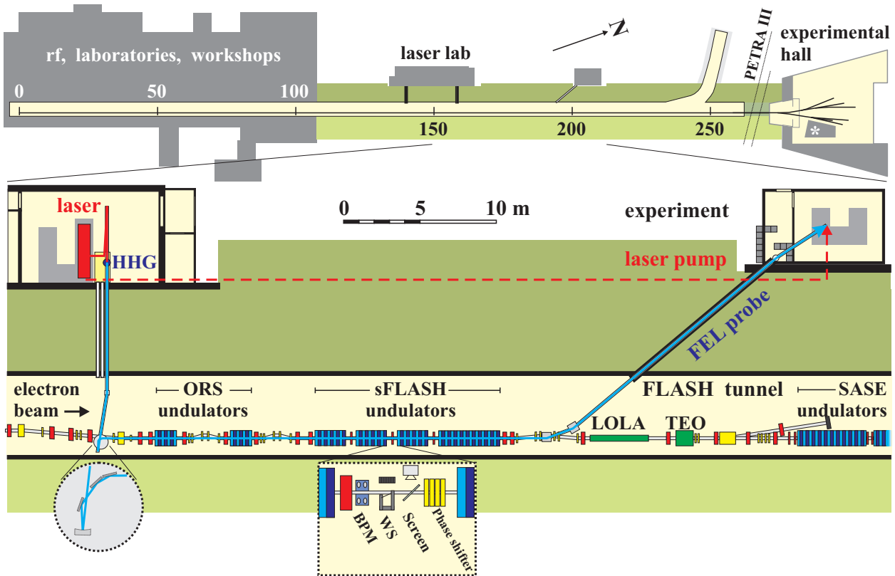
Figure 1: The FLASH facility (top) is comprised of a 260m long tunnel housing the linac and the SASE-undulators, followed by an experimental hall. sFLASH is located in the section upstream of the SASE-undulators. Seed pulses from the HHG source in the building adjacent to the FLASH tunnel are injected into the electron beam pipe downstream of the last dipole of the energy collimator (left). By means of an IR-beamline (dashed red line), a fraction of the optical drive laser energy can be used for pump-probe experiments. The dashed bordered boxes show detailed views of the XUV-injection and the undulator intersections.
