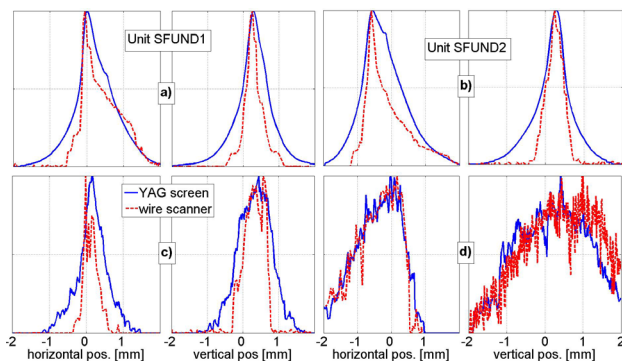
Figure 4: Electron beam profiles (upper row a) and b)) and XUV-laser beam profiles (lower row c) and d)) each measured with cerium-doped YAG screens and EMCCD cameras (blue lines) and with wire scanners (red lines) after adjusting the transverse laser position. The profile intensity is normalized to the same peak value for each measurement.
