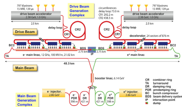
Figure 1: Conceptual layout of CLIC.
