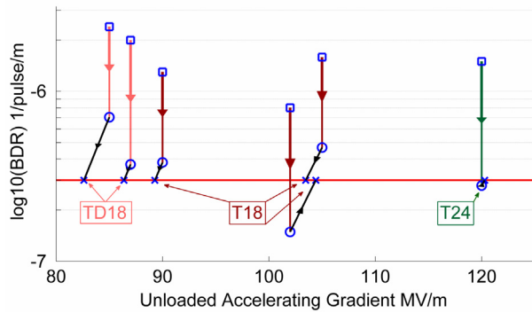
Figure 2: Gradient and breakdown rate achieved with different CLIC structures [4]. The actual measurements are marked with squares, the expected breakdown rate for the nominal pulse length with circles and the expected gradient for the nominal breakdown rate with crosses.
