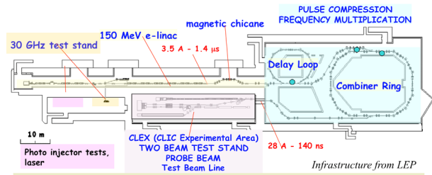
Figure 3: Layout of CTF3.
