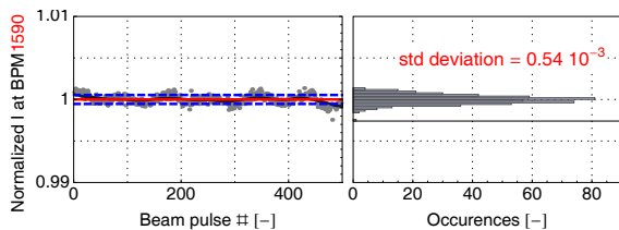
Figure 5: Pulse current variation measured at the end of the CTF3 drive beam linac.
