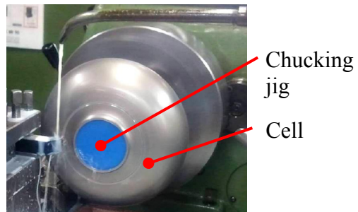
Figure 8: Image of new thinning process of cell.
