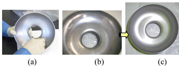
Figure 7: Finishing for inner surface of cell. (a) Present status (Finishing by human hand), (b) Seamless dumbbell before finishing, (c) Seamless dumbbell after finishing by robot
