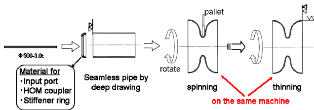
Figure 6: Flow of seamless dumbbell.
