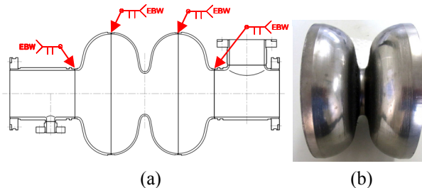
Figure 5: (a) Over view of MHI-B cavity, (b) Seamless dumbbell.
