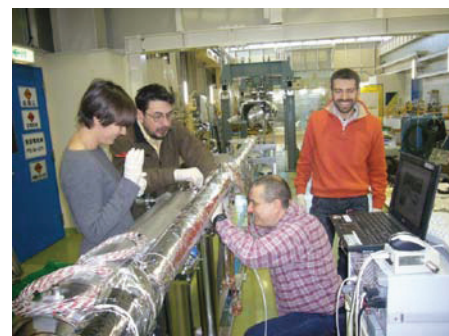
Figure 1: String assembly of four TESLA-type cavities by DESY/FNAL/KEK team (top), and tuner assembly by INFN/FNAL team (bottom).
