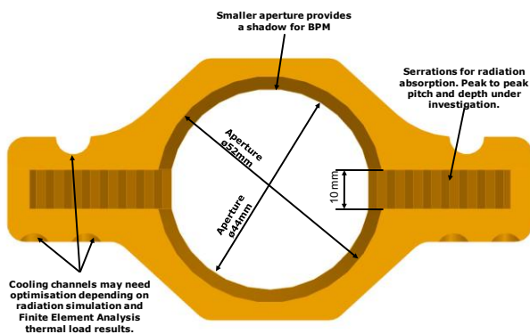
Figure 3: SR power absorber.
