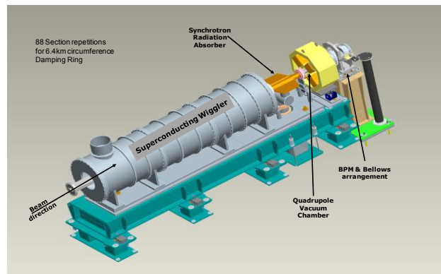
Figure 1: Layout of the ILC DR wiggler module.
