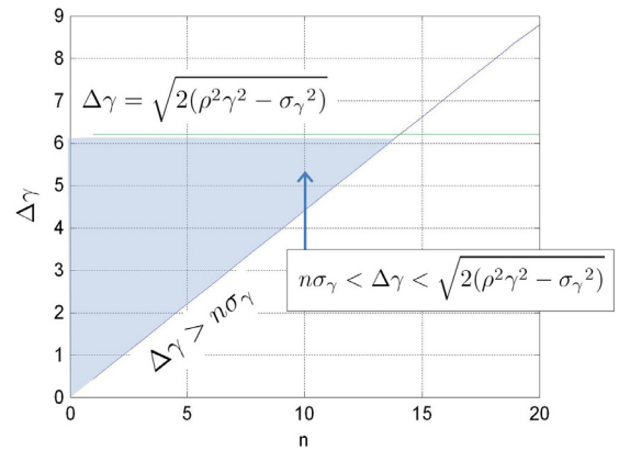
Figure 6: Energy modulation criteria for successful FEL operation, as a function of harmonic number.
