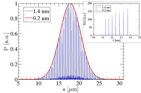
Figure 4: Normalised longitudinal profile, and spectrum (inset), of the input seed for the two cases of filtering.
