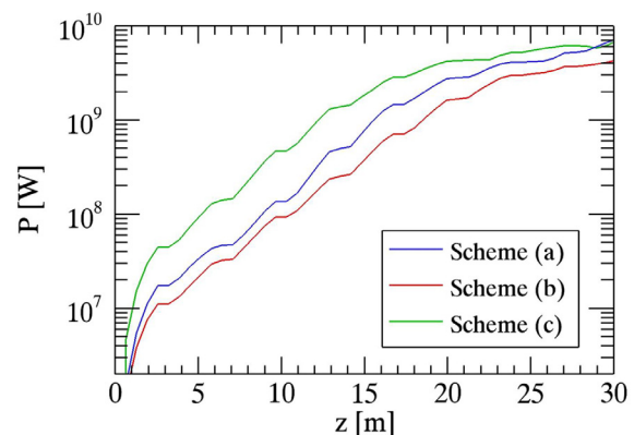
Figure 2: Radiation power as a function of distance through the radiator for time-dependent Genesis 1.3 simulations of the three modulator configurations
