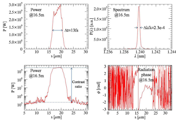
Figure 3: Start-to-end FEL simulation results for FEL-3 operating at 1 keV photon energy at saturation. Top left shows the longitudinal profile of the radiation power and top right shows the spectrum. Bottom left shows a log plot of the power profile to assess the contrast ratio and bottom right shows the radiation phase. The contrast ratio is \approx 12500 and time bandwidth product \Delta\nu\Delta t \approx 0.77 .
