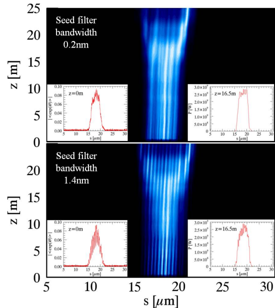
Figure 5: Evolution of the normalised longitudinal radiation profile with distance through the radiator. Also shown is the bunching at the start of the radiator (inset left), and radiation profile at saturation (inset right).
