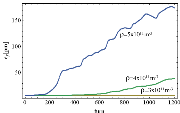
Figure 1: Emittance growth due to the single-bunch instability caused by the electron cloud effect.
