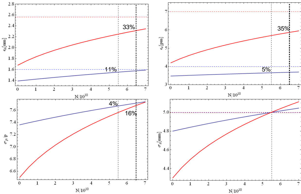
Figure 2: Transverse emittance growth, and growth in bunch length and energy spread in the SuperB LER (red) and HER (blue), as functions of the bunch charge.
