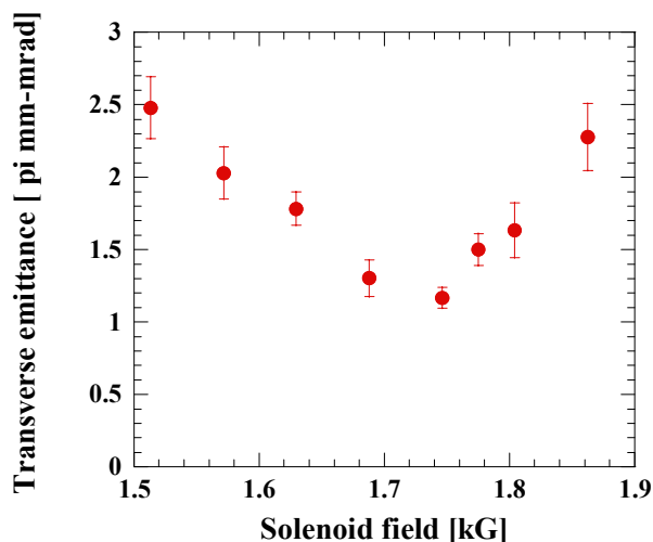
Figure 3: Emittance at the linac exit as a function of magnetic field of the solenoid. The laser injection phase and the bunch charge were 25^\circ and 50 pC/pulse, respectively.
