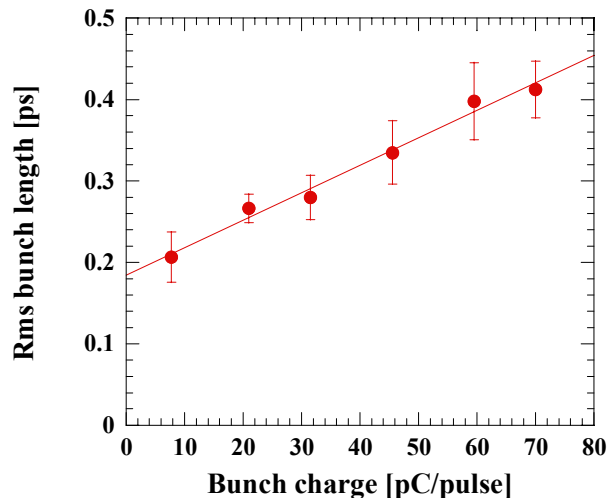
Figure 4: Rms bunch length as a function of bunch charge. The bunch charge was varied by changing the driving laser power of the regenerative amplifier.
