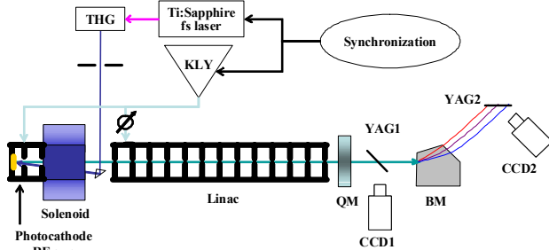
Figure 1: Schematic diagram of a femtosecond electron source.
