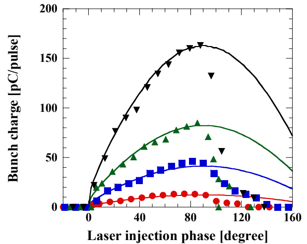
Figure 2: Bunch charge as a function of injection phase of the femtosecond UV light. The UV power were 3 (circle), 10 (square), 20 (uptriangle) and 40 (downtriangle) \mu\text{J}/\text{pulse} from the bottom.
