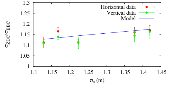
Figure 2: Ratio of the ZDC and BBC beam sizes as measured from the Vernier scans. \sigma_s represents the convoluted bunch length.
