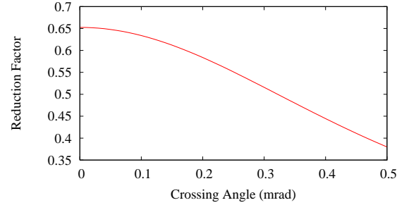
Figure 3: Reduction factor due to the combined effect of the crossing angle and the hourglass effect for \sigma_s = 1 m and \beta^* = 0.7 m.
