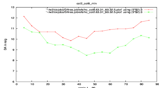
Figure 6: DA limited by IT multipole errors: green: compensation of b3 and b6, red: correction of a3, b3, a4, b4, b6 (no D1 errors included).
