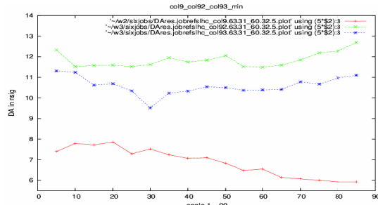
Figure 9: Resume: Dynamic aperture obtained for the original error table with and without corrector scheme (red and blue curve), and the result of improved multipole coefficients (green).
