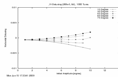
Figure 3: Detuning in the horizontal plane under the influence of strong nonlinear multipole fields of the new low- \beta quadrupole MQXC.
