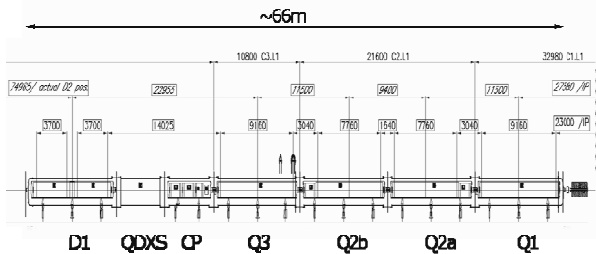
Figure 1: The new LHC interaction region
