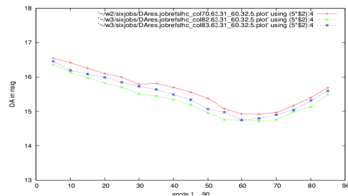
Figure 7: Probing the effect of single multipole fields.
