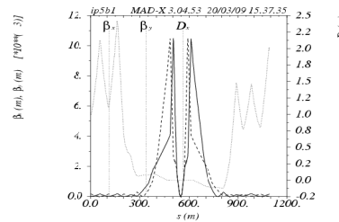
Figure 2: Beam optics in IR 1 for the upgrade LHC
