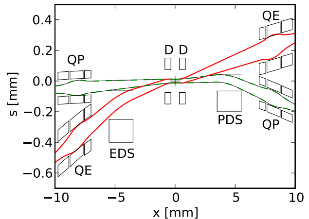
Figure 1: A sketch of the ENC IR region. Red solid line ...electrons, green dashed lines ...protons. large cross ...IP. Magnets: D ...separation dipole, PDS ...spectrometer dipole, EDS ...electron spectrometer dipole; QP ...proton triplet quadrupole, QE ...electron triplet quadrupole.
