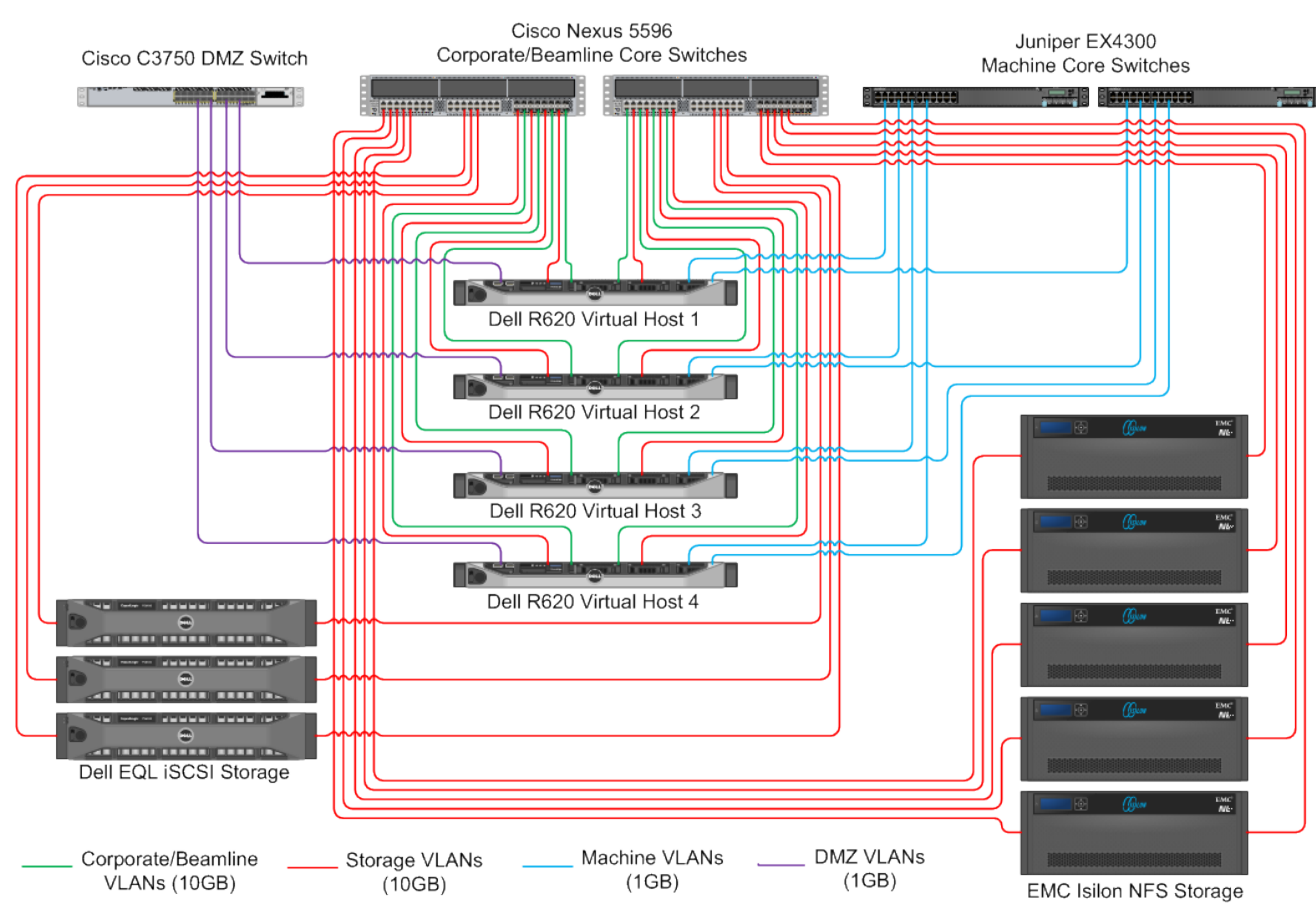
Virtualisation Platform of the Australian Synchrotron. Not shown are the separate backup systems for the iSCSI and the NFS storage systems.
