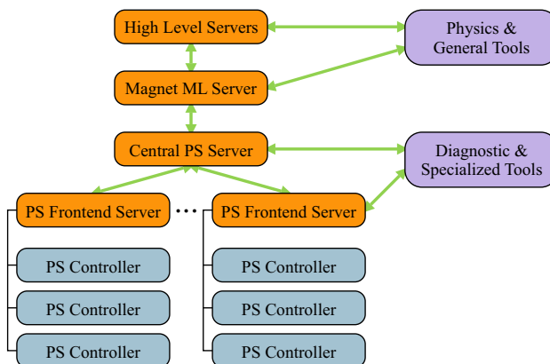
Figure 1: An overview of communication paths between user tools, various server layers, and power supply controller hardware.
