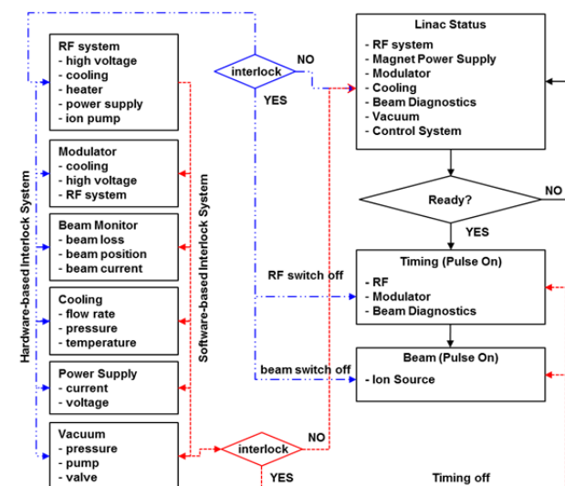
Figure 2: Block diagram of interlock system for machine protection with hardware and software based interlock system.
