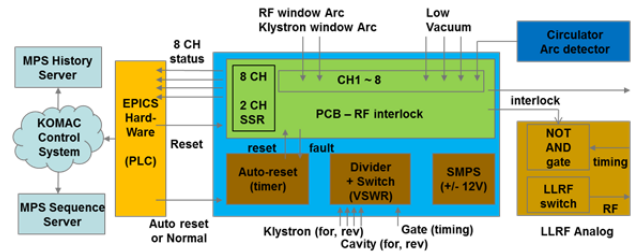
Figure 3: Block diagram of the signal path of interlock system developed by using a fast trip direct analogue circuit.
