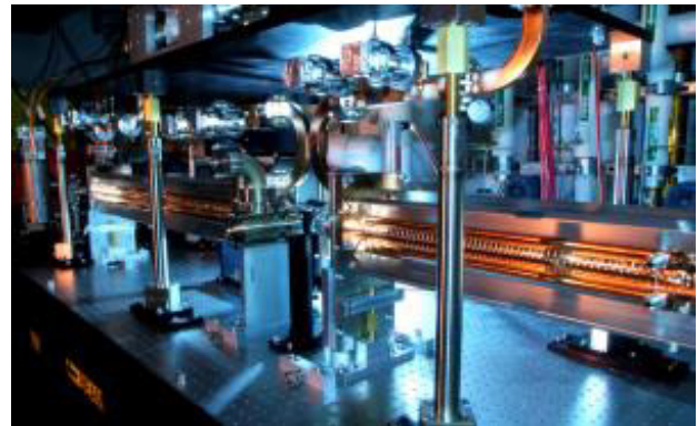
Figure 2: Two one-meter long X-Band RF structures are in the beamline's path towards the e-beam dump. (Image: P. Krejcik/SLAC).
