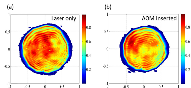
Figure 3: Transverse laser profile at virtual cathode with the laser used only (a) and with the AOM inserted (b).
