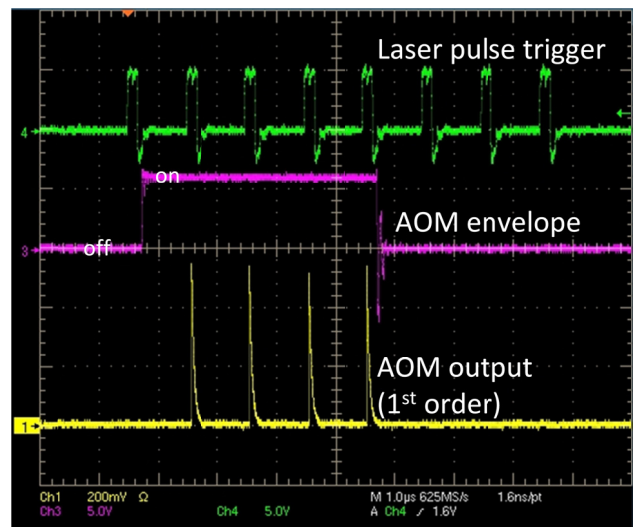
Figure 2: Pulse selection with AOM. Upper trace: laser pulse trigger at 1 MHz repetition frequency. Middle trace: AOM control envelope. Lower trace: AOM output.
