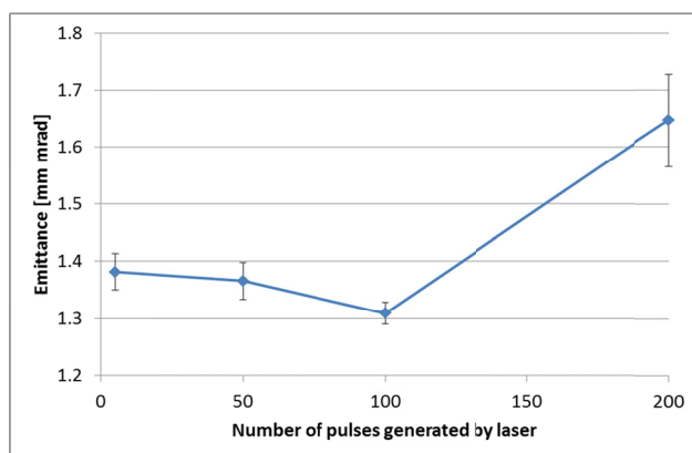
Figure 7: X-Emittance measured vs. number of laser pulses. Error bars show statistical error.
