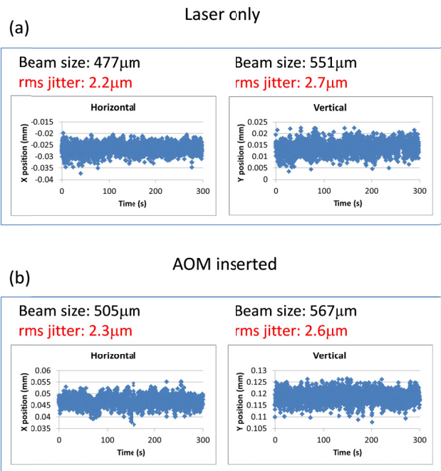
Figure 5: Laser pointing stability with the laser used only (a) and with the AOM inserted (b).
