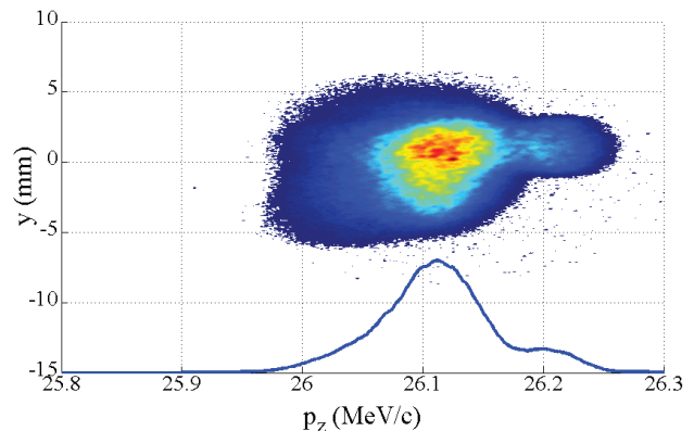
Figure 4: Electron beam image measured at the first screen of the second dispersive arm. Horizontal axis corresponds to the longitudinal momentum distribution.
